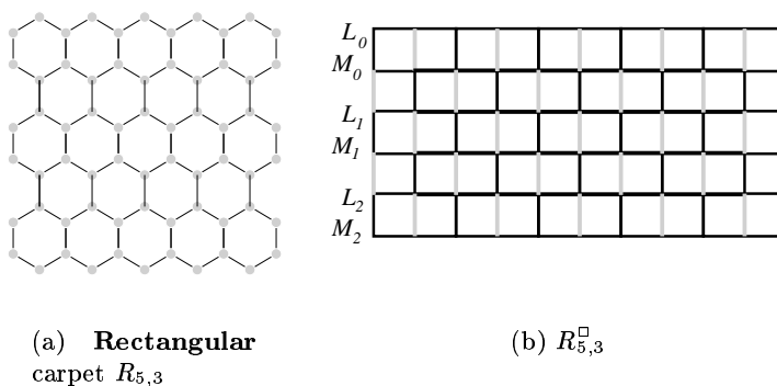
Figure 9: A Rectangular Carpet
