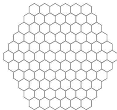
Figure 14: Crown of Order 6
