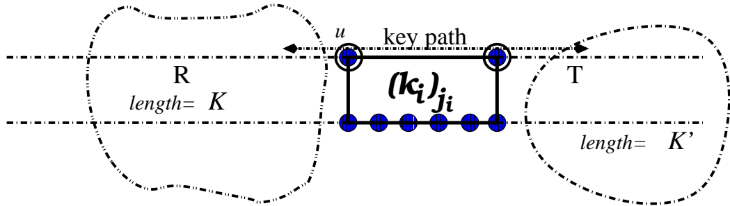
Figure 3: Changes after one rotation
