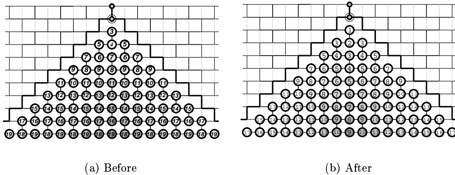
Figure 10: Effects of Squaring on distances in carpets
