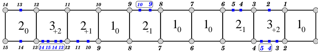
Figure 6: A Chain with many Turns: \mathcal{X} = q(q+1) \left( \frac{q^{14} - 1}{q-1} + q^{12} \frac{q^2 - 1}{q-1} + q^8 + q^3 \right)
