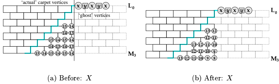
Figure 11: “Edge Effects”, as seen before and after the squaring
