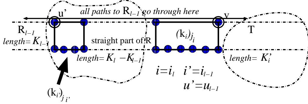
Figure 4: The two Segments of R
