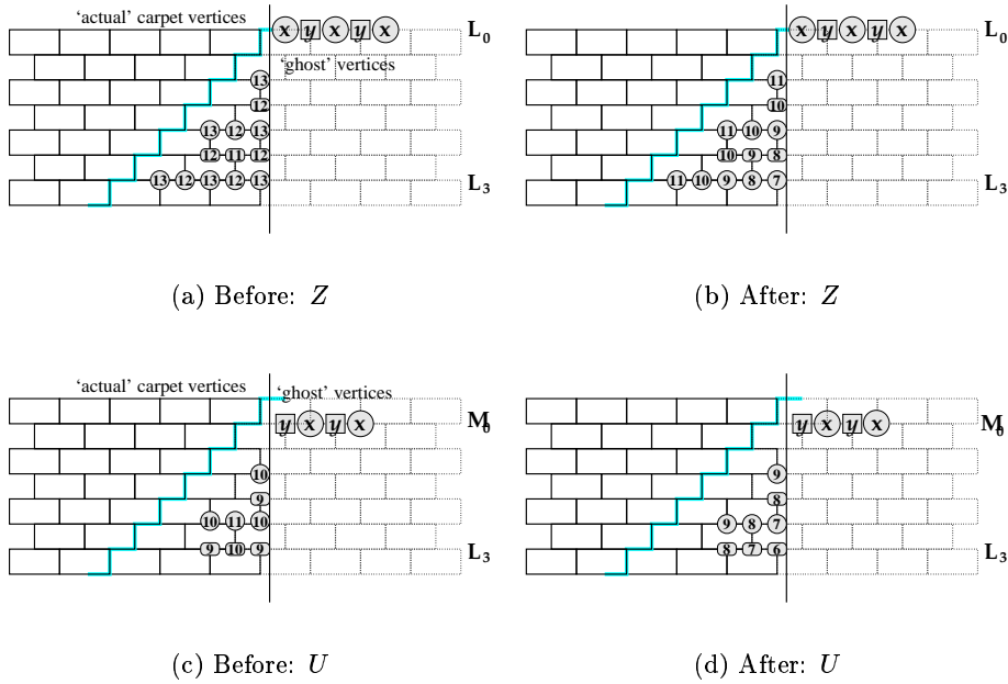
Figure 13: The two other “Edge Effects”, before and after the squaring
