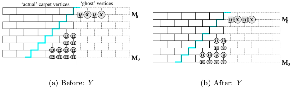
Figure 12: A different “Edge Effect”, as seen before and after the squaring
