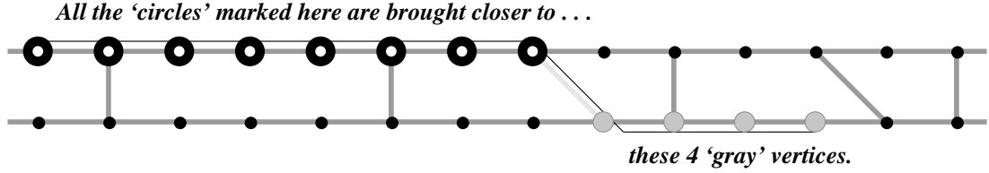
(b) Process of subdivision
